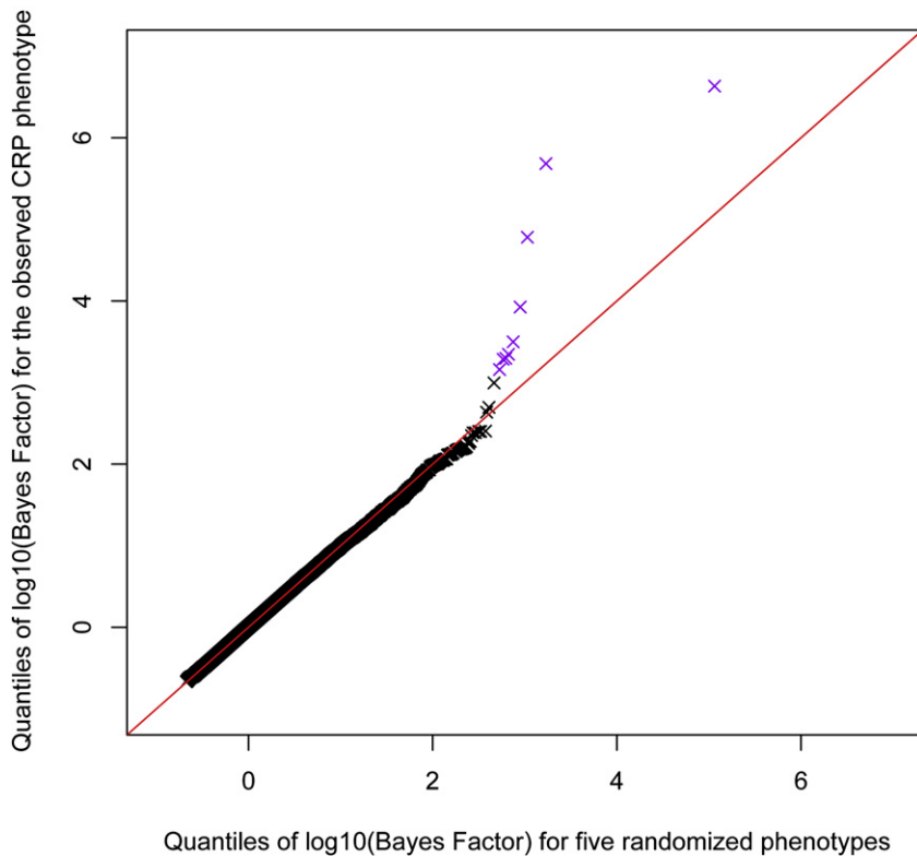
Figure 1. Distribution of Bayes Factors Associated with C-Reactive Protein in Stage 1 of PARC Genome-wide Association Study
